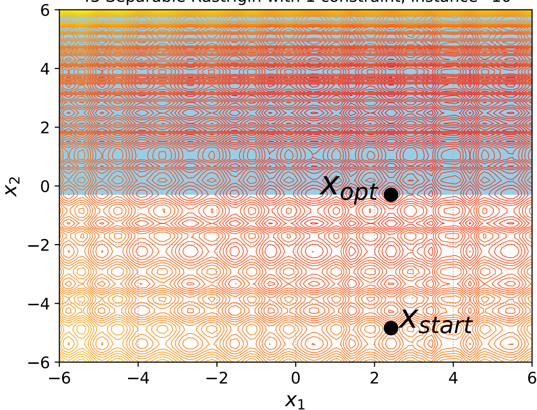
43 Separable Rastrigin with 1 constraint, instance=10
