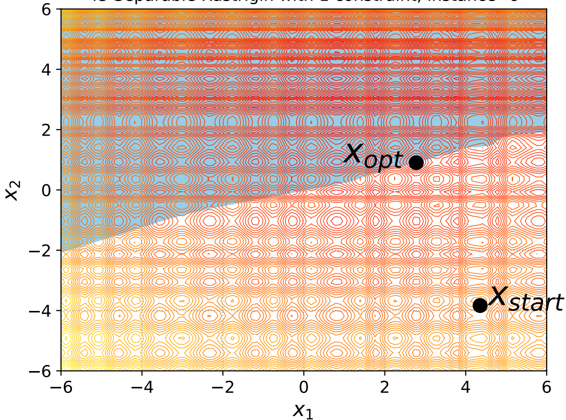
43 Separable Rastrigin with 1 constraint, instance=9
