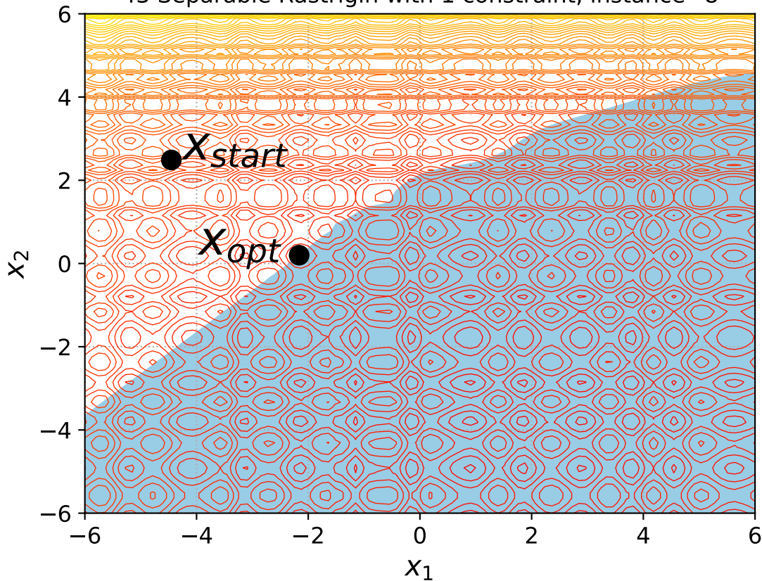
43 Separable Rastrigin with 1 constraint, instance=8
