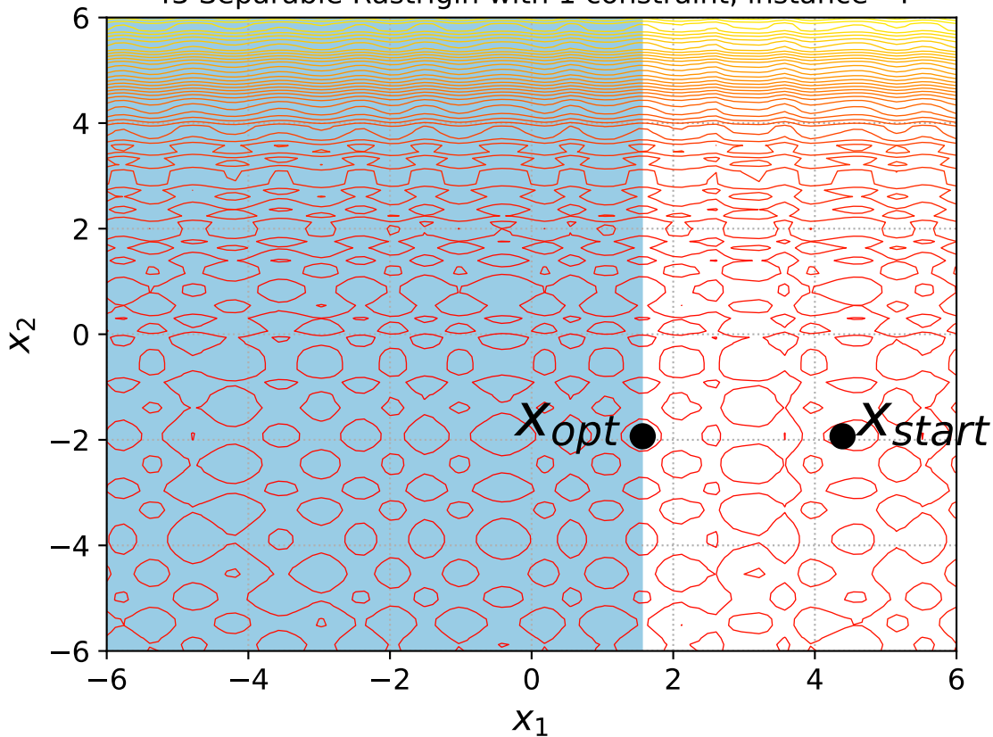
43 Separable Rastrigin with 1 constraint, instance=4
