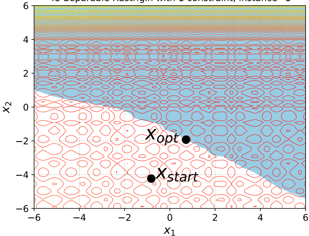
43 Separable Rastrigin with 1 constraint, instance=1
