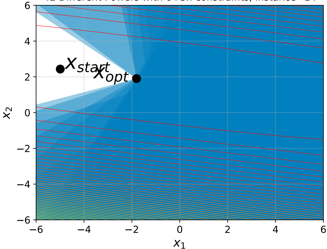
42 Different Powers with 6+3n constraints, instance=14
