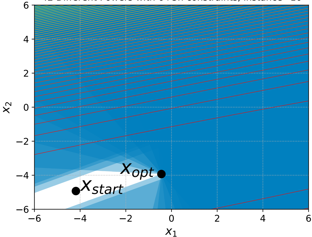
42 Different Powers with 6+3n constraints, instance=10
