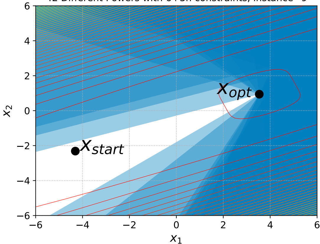
42 Different Powers with 6+3n constraints, instance=9
