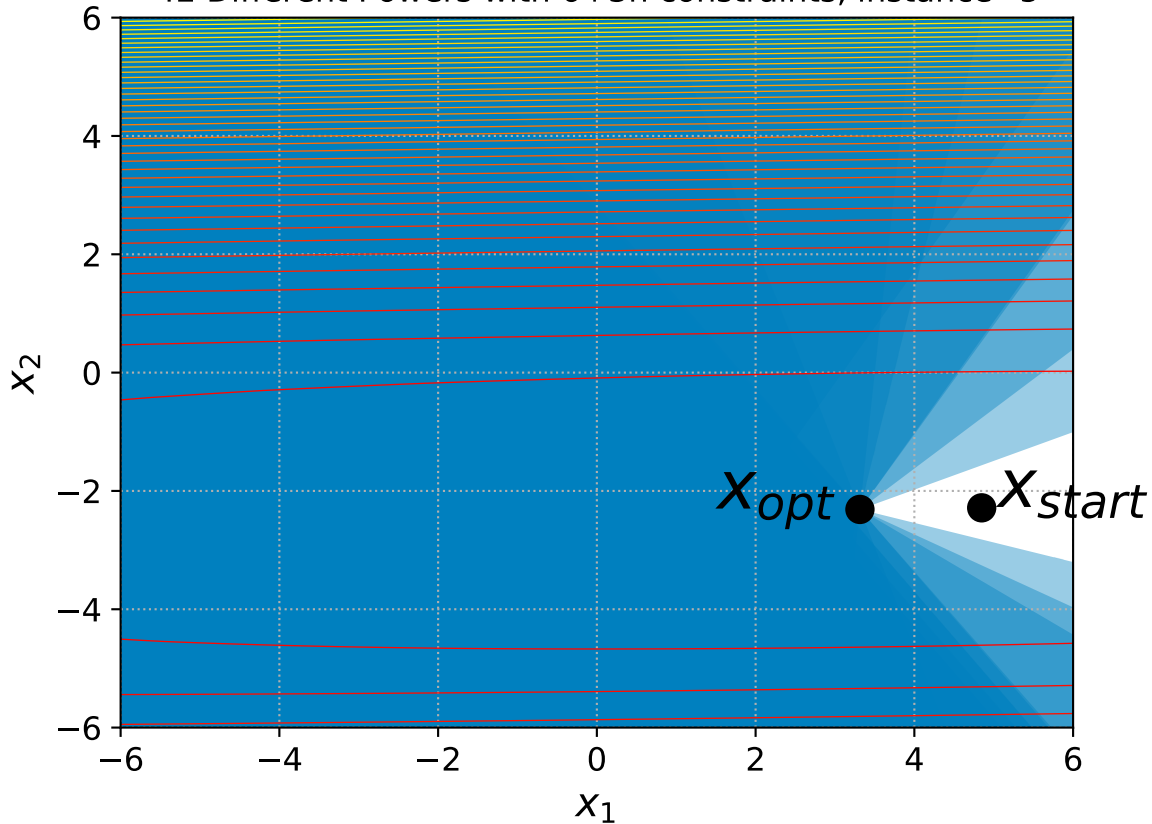
42 Different Powers with 6+3n constraints, instance=5
