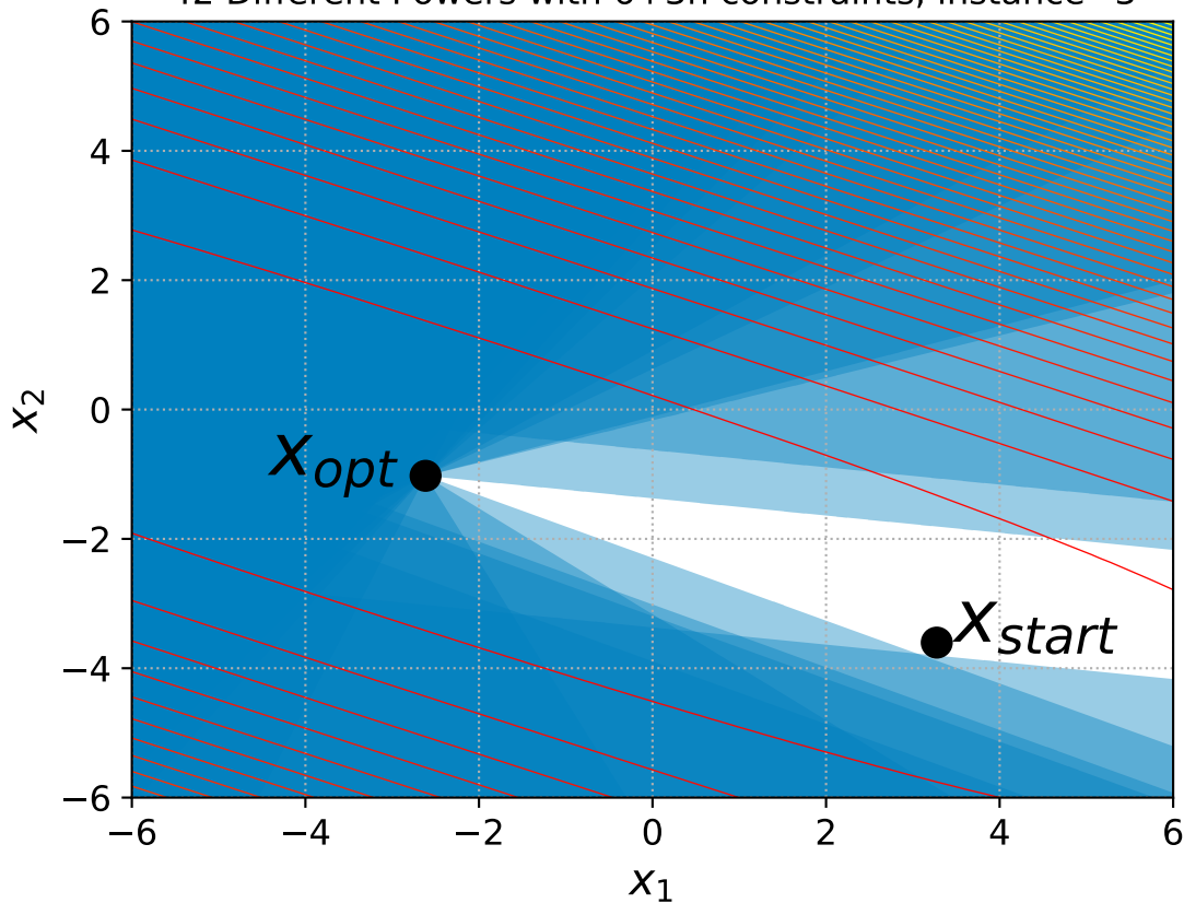
42 Different Powers with 6+3n constraints, instance=3
