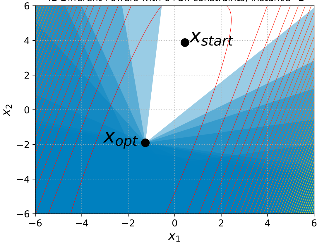
42 Different Powers with 6+3n constraints, instance=2
