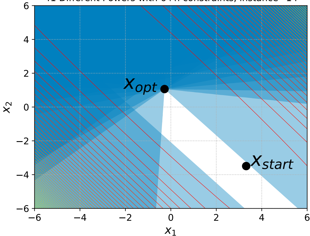
41 Different Powers with 6+n constraints, instance=14
