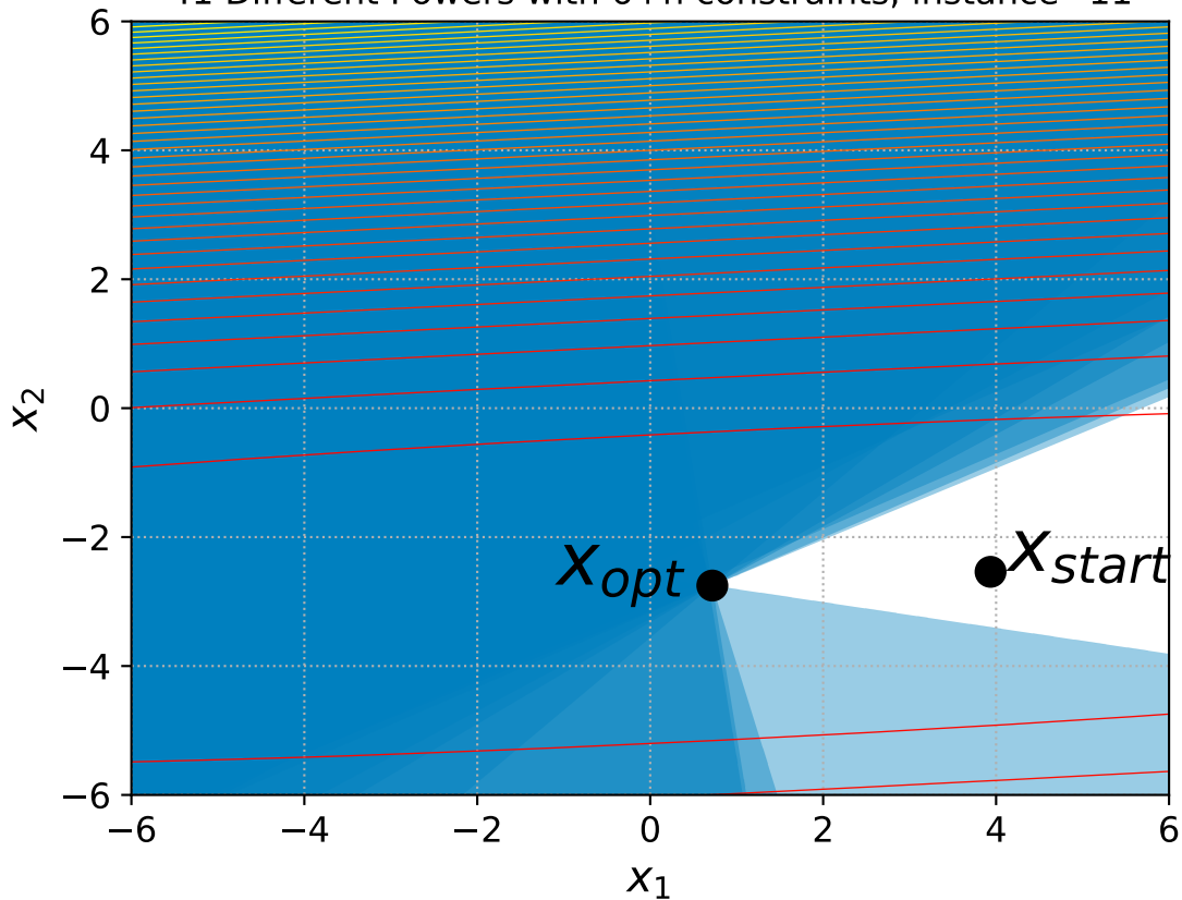
41 Different Powers with 6+n constraints, instance=11
