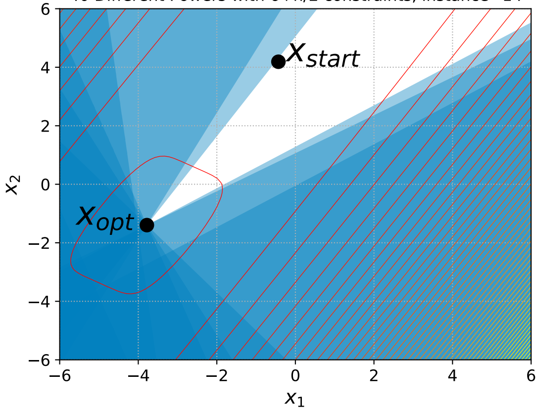
40 Different Powers with 6+n/2 constraints, instance=14
