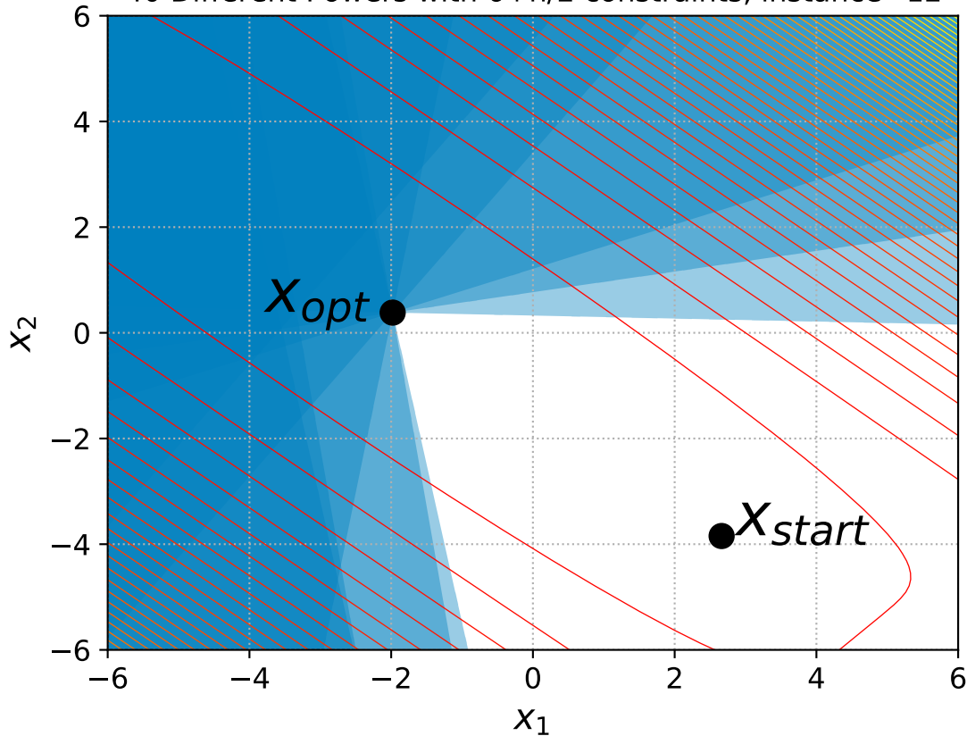
40 Different Powers with 6+n/2 constraints, instance=12
