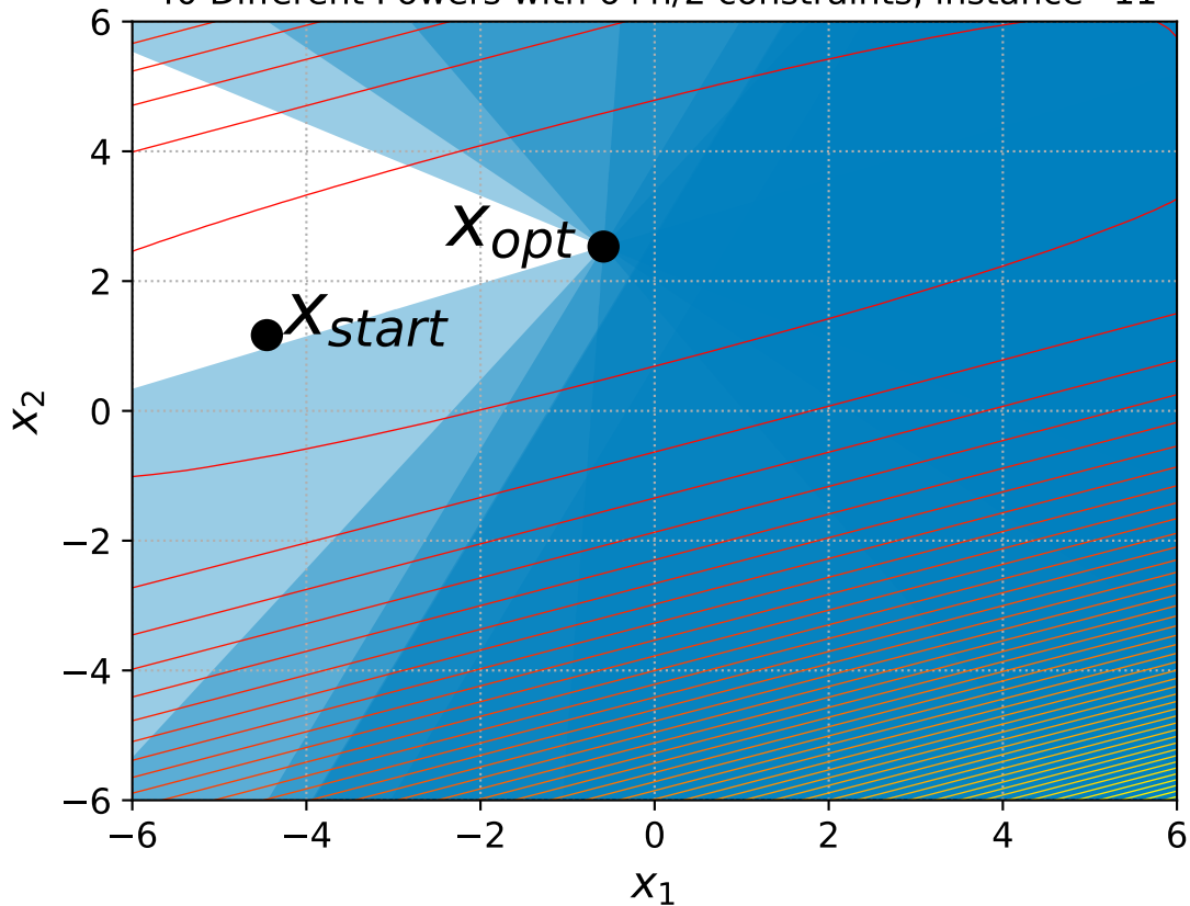
40 Different Powers with 6+n/2 constraints, instance=11
