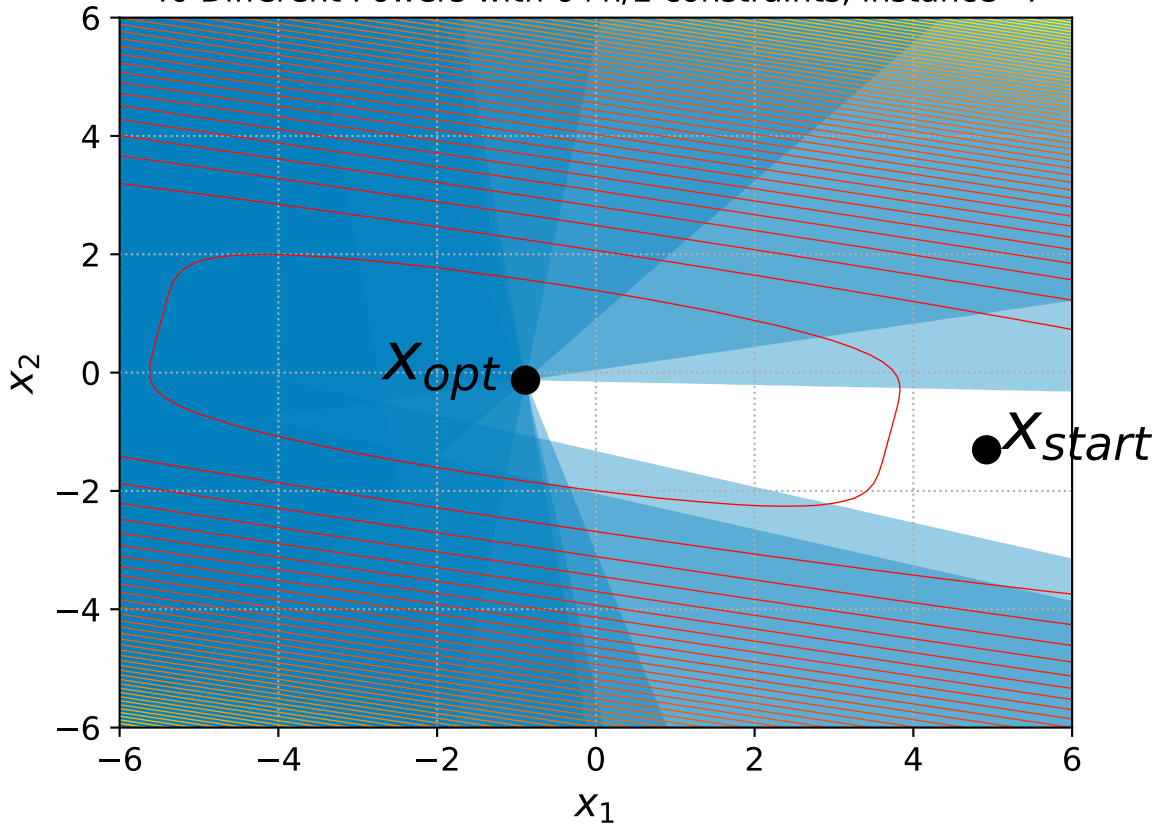
40 Different Powers with 6+n/2 constraints, instance=7
