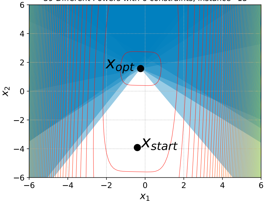
39 Different Powers with 6 constraints, instance=13
