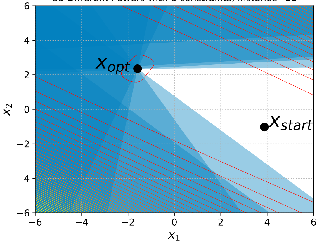
39 Different Powers with 6 constraints, instance=11
