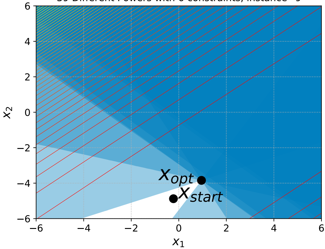
39 Different Powers with 6 constraints, instance=9
