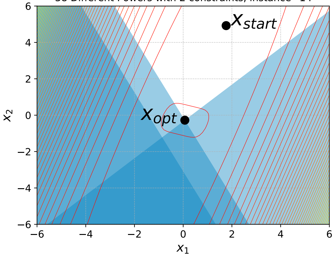
38 Different Powers with 2 constraints, instance=14
