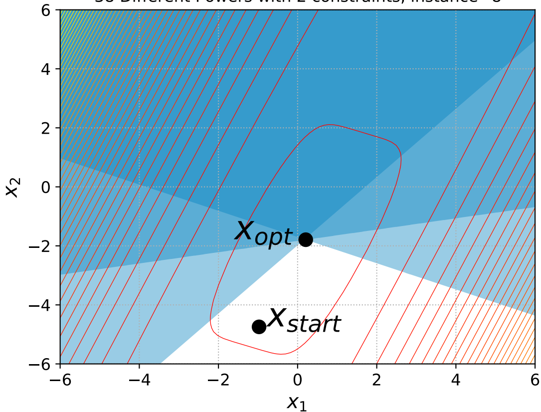
38 Different Powers with 2 constraints, instance=8
