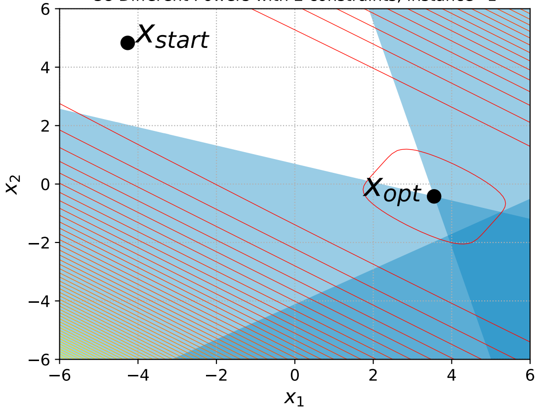
38 Different Powers with 2 constraints, instance=1
