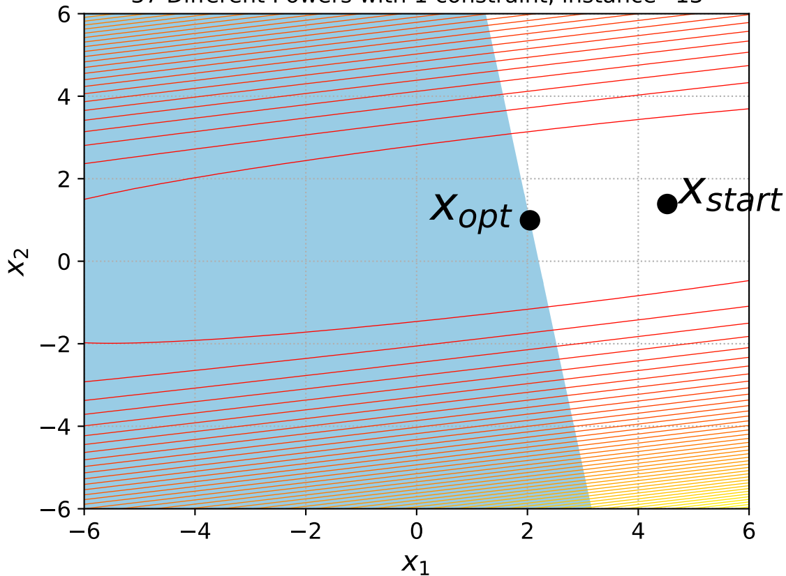
37 Different Powers with 1 constraint, instance=13
