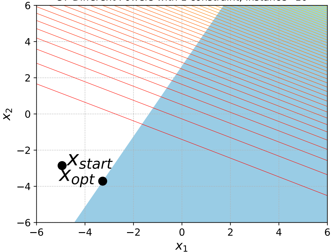
37 Different Powers with 1 constraint, instance=10
