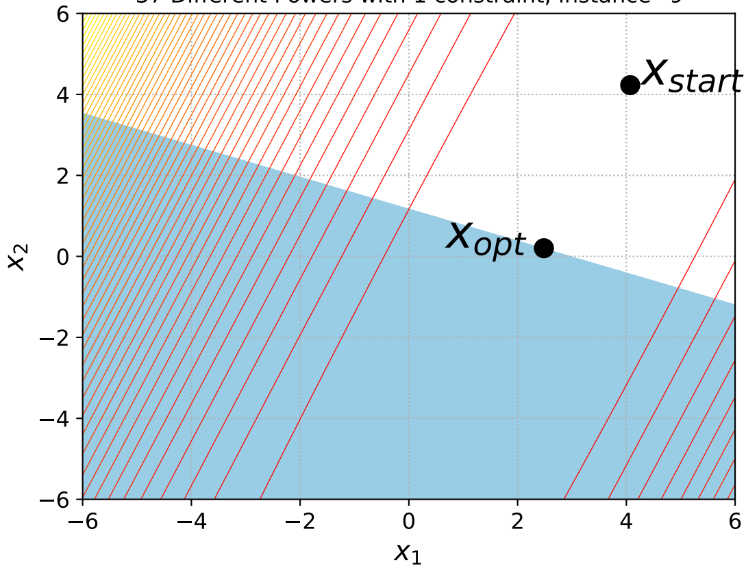
37 Different Powers with 1 constraint, instance=9
