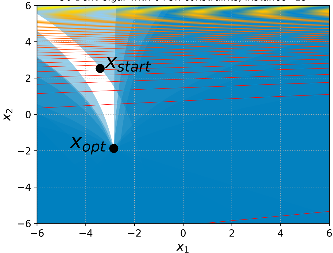
36 Bent Cigar with 6+3n constraints, instance=13
