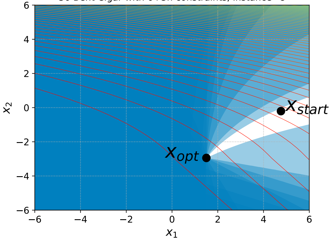
36 Bent Cigar with 6+3n constraints, instance=8
