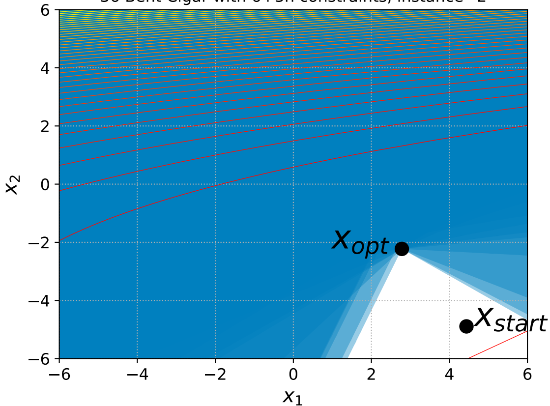
36 Bent Cigar with 6+3n constraints, instance=2
