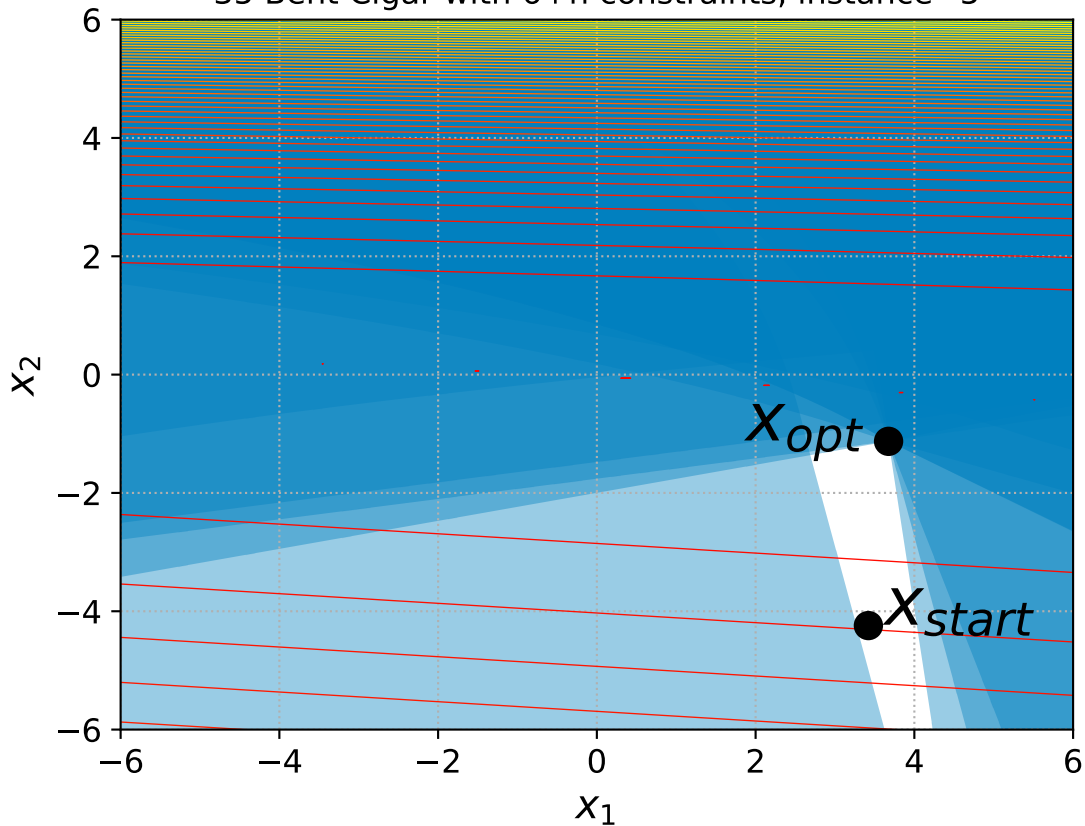
35 Bent Cigar with 6+n constraints, instance=5
