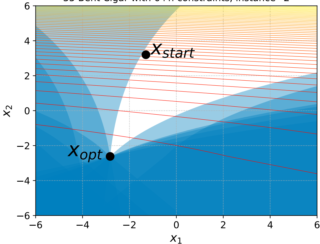
35 Bent Cigar with 6+n constraints, instance=2
