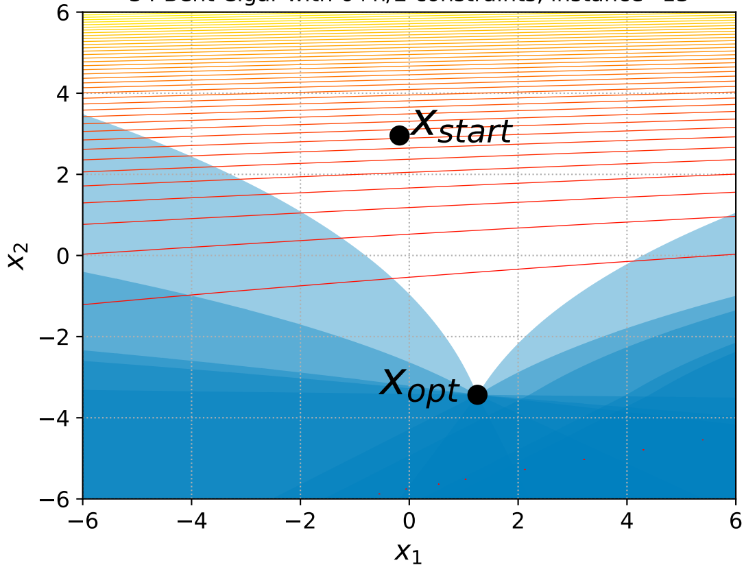
34 Bent Cigar with 6+n/2 constraints, instance=13
