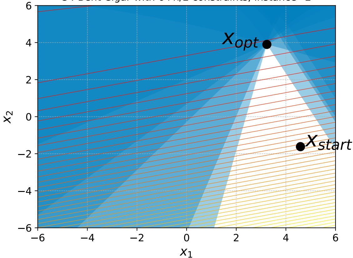
34 Bent Cigar with 6+n/2 constraints, instance=2
