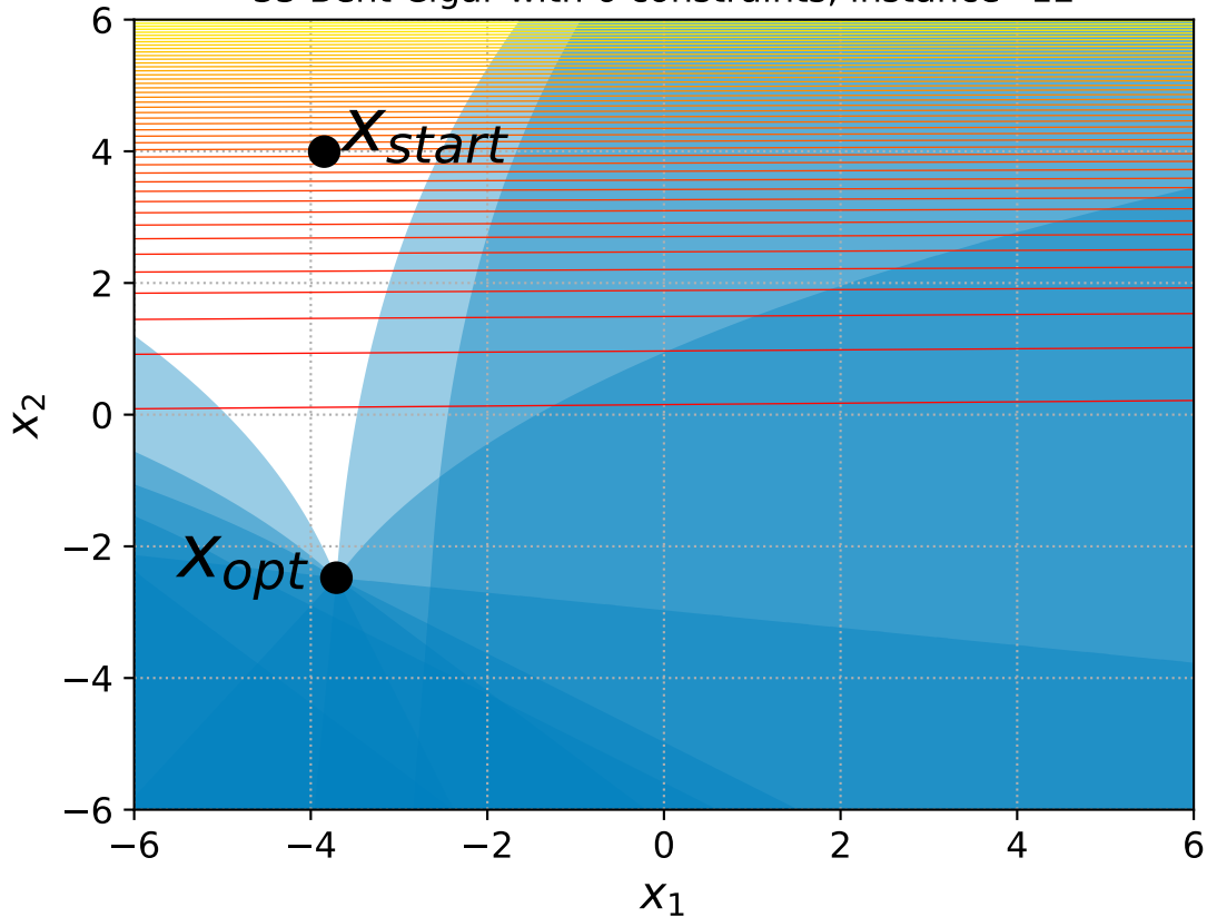
33 Bent Cigar with 6 constraints, instance=12
