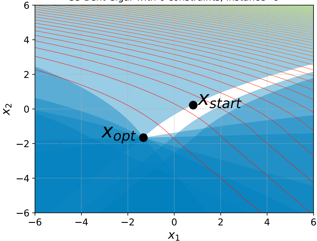
33 Bent Cigar with 6 constraints, instance=9
