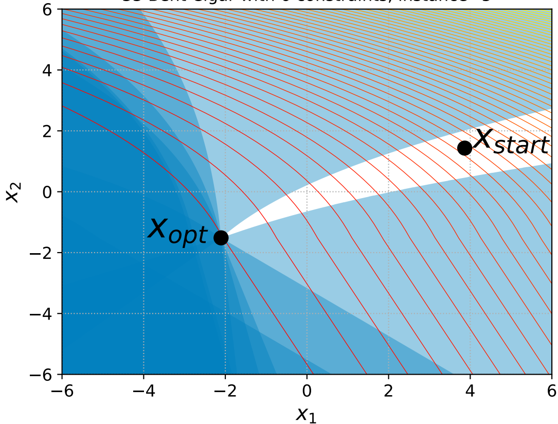
33 Bent Cigar with 6 constraints, instance=5
