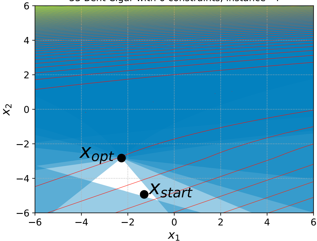
33 Bent Cigar with 6 constraints, instance=4
