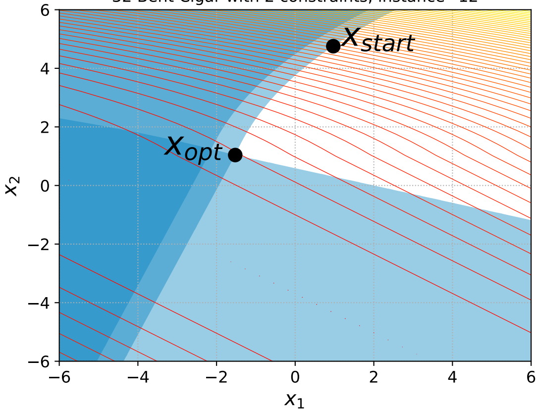
32 Bent Cigar with 2 constraints, instance=12
