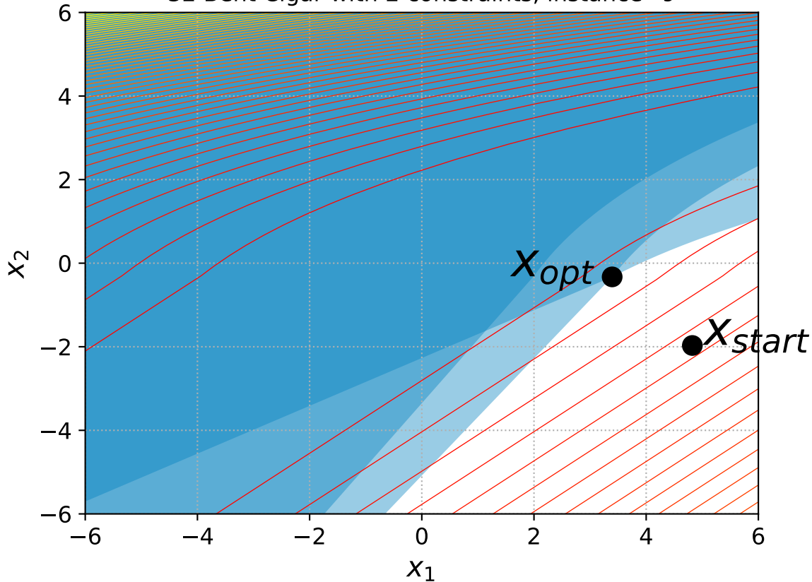
32 Bent Cigar with 2 constraints, instance=9
