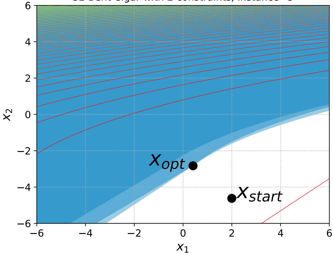
32 Bent Cigar with 2 constraints, instance=3
