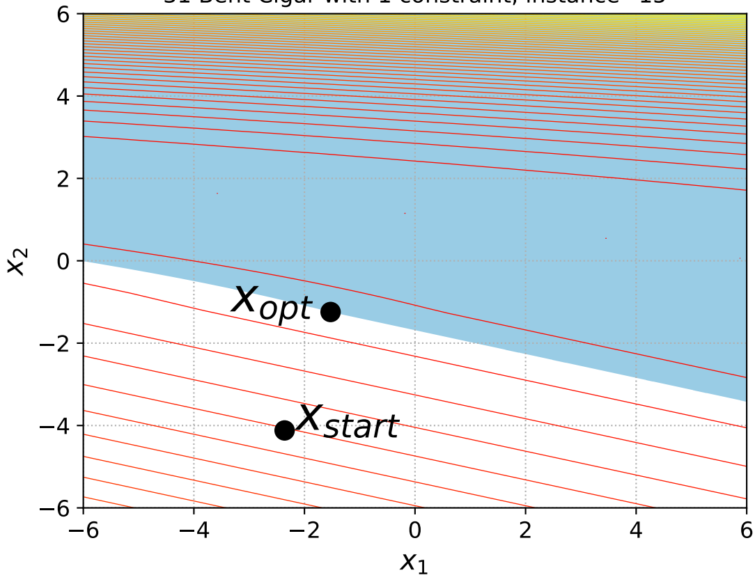
31 Bent Cigar with 1 constraint, instance=15
