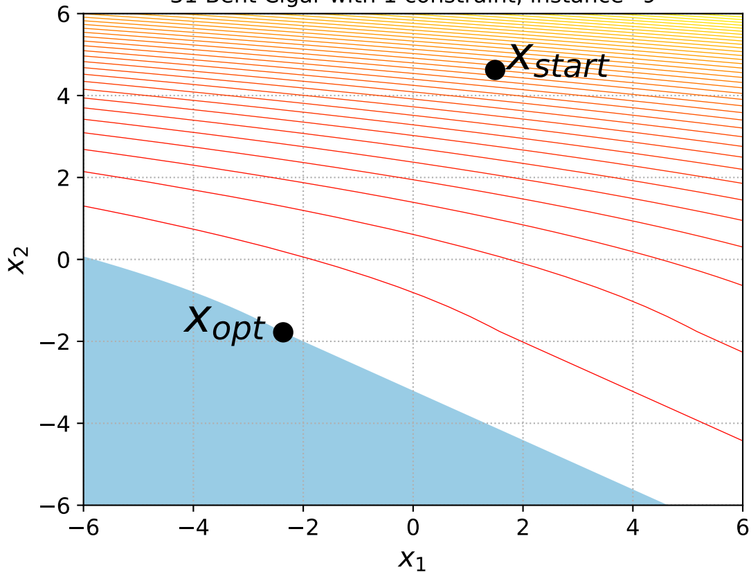
31 Bent Cigar with 1 constraint, instance=9
