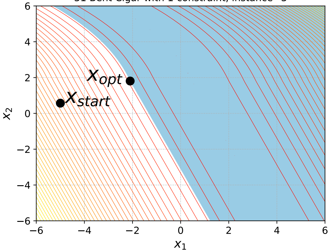
31 Bent Cigar with 1 constraint, instance=3
