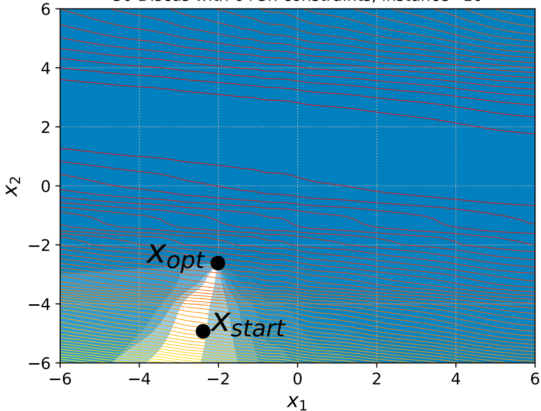
30 Discus with 6+3n constraints, instance=10
