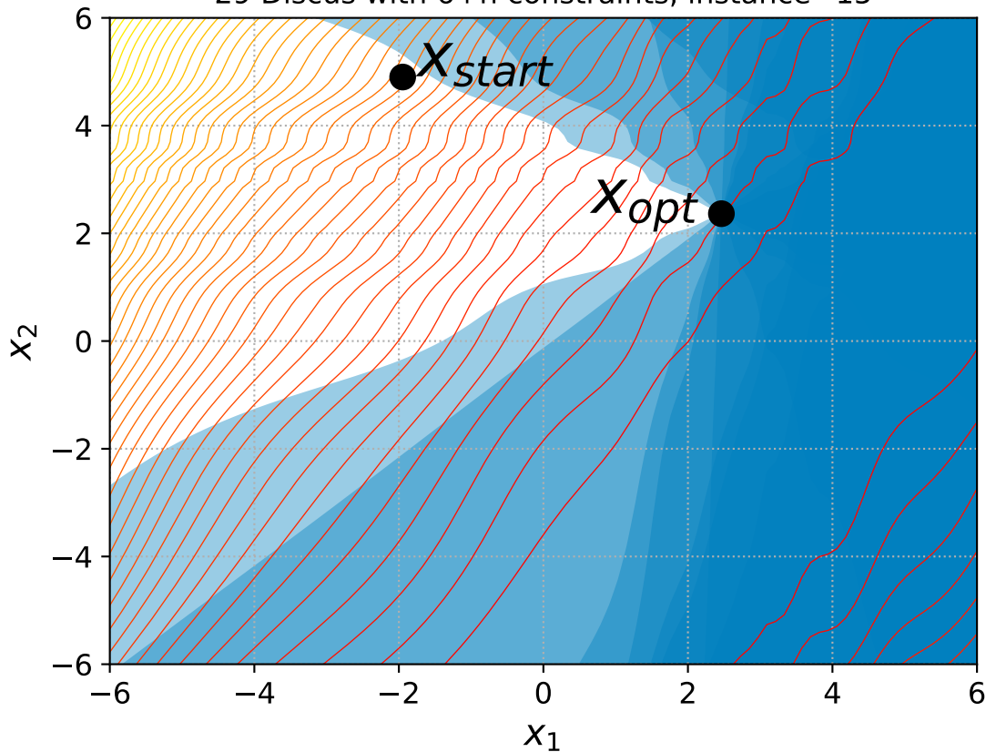
29 Discus with 6+n constraints, instance=15
