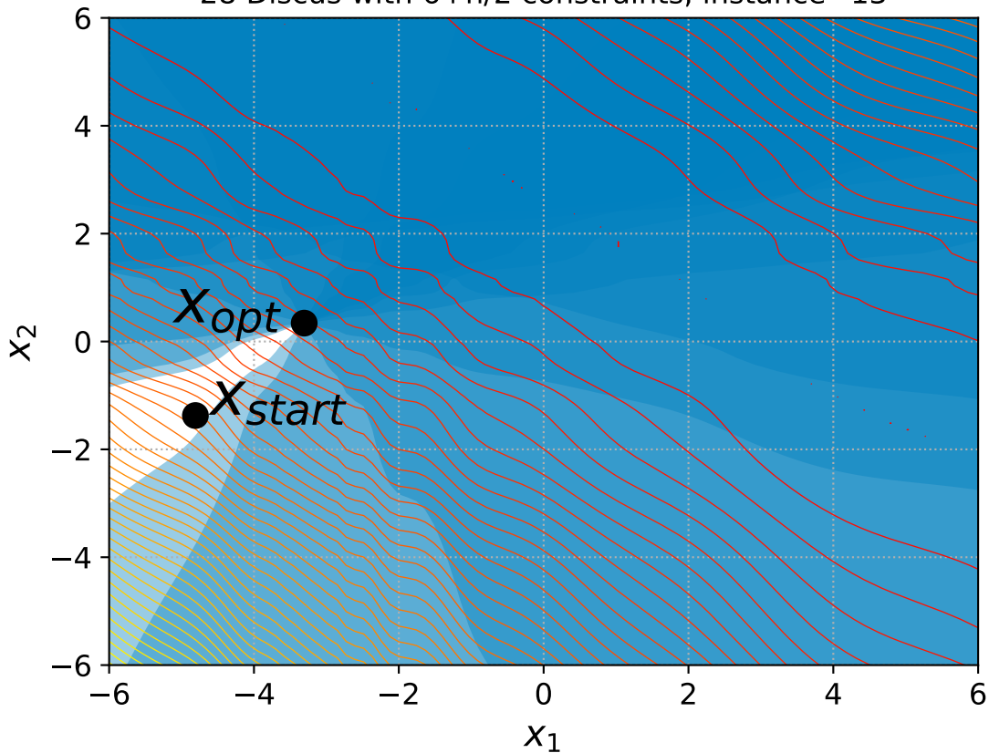
28 Discus with 6+n/2 constraints, instance=13
