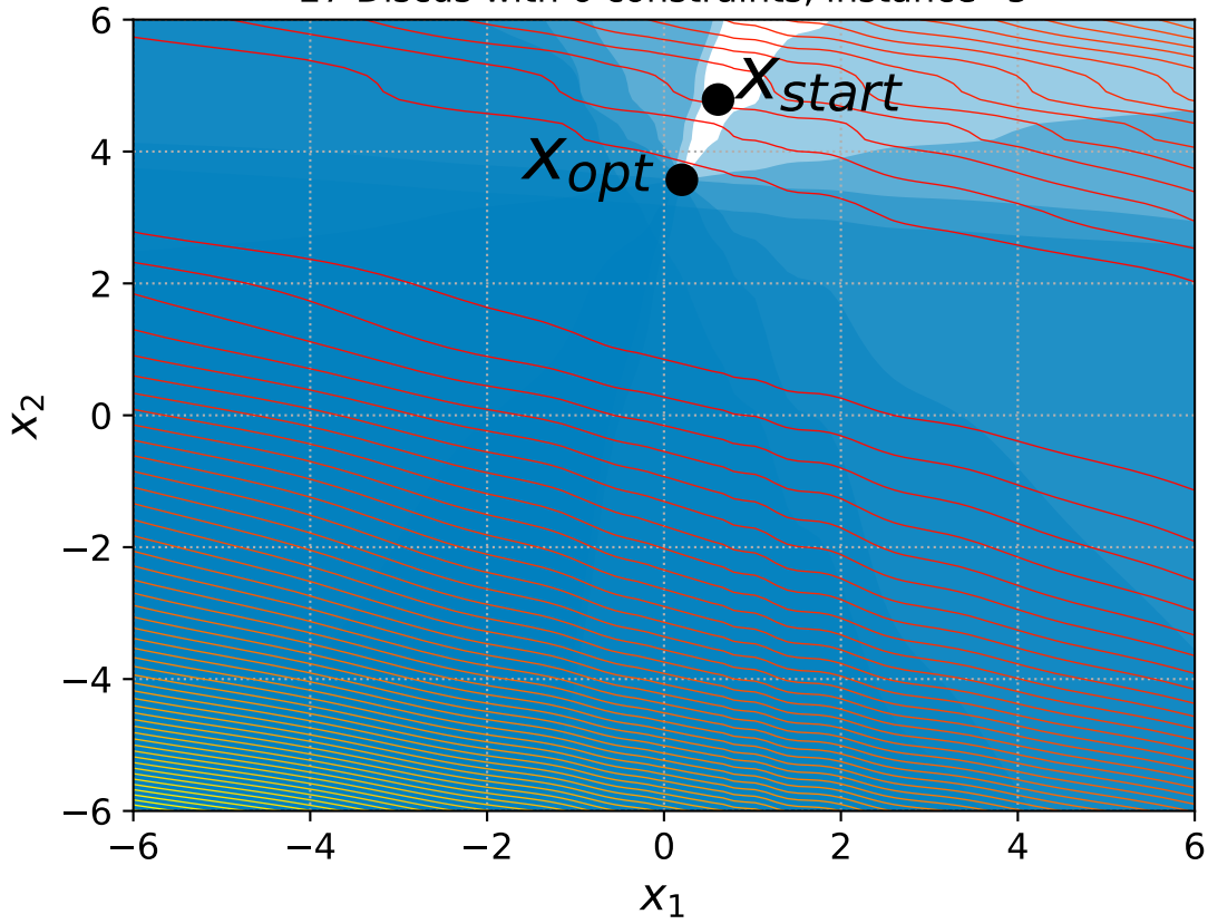
27 Discus with 6 constraints, instance=5
