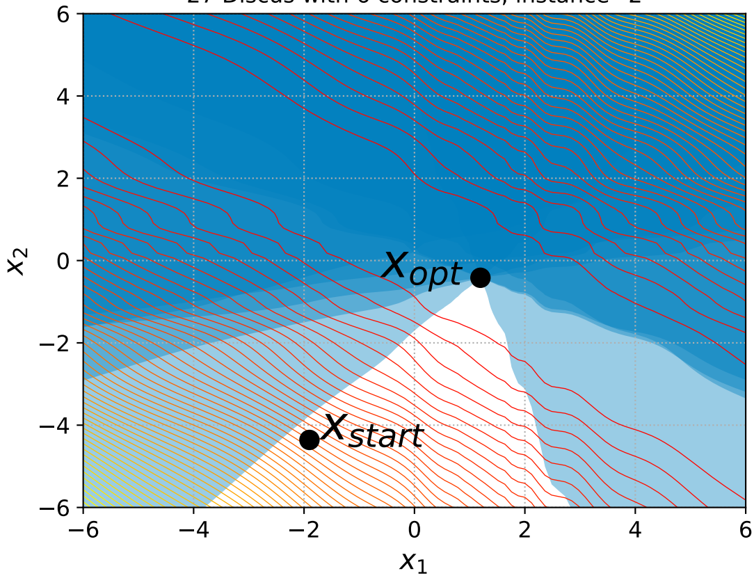
27 Discus with 6 constraints, instance=2
