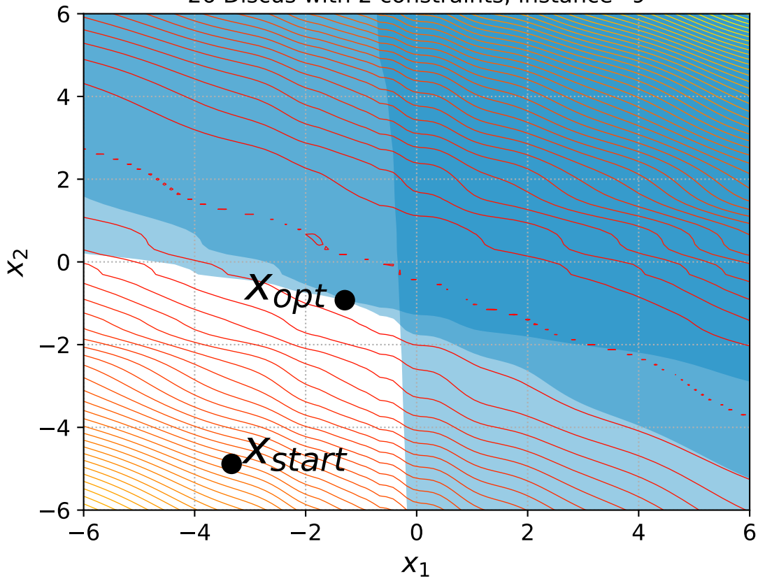
26 Discus with 2 constraints, instance=9
