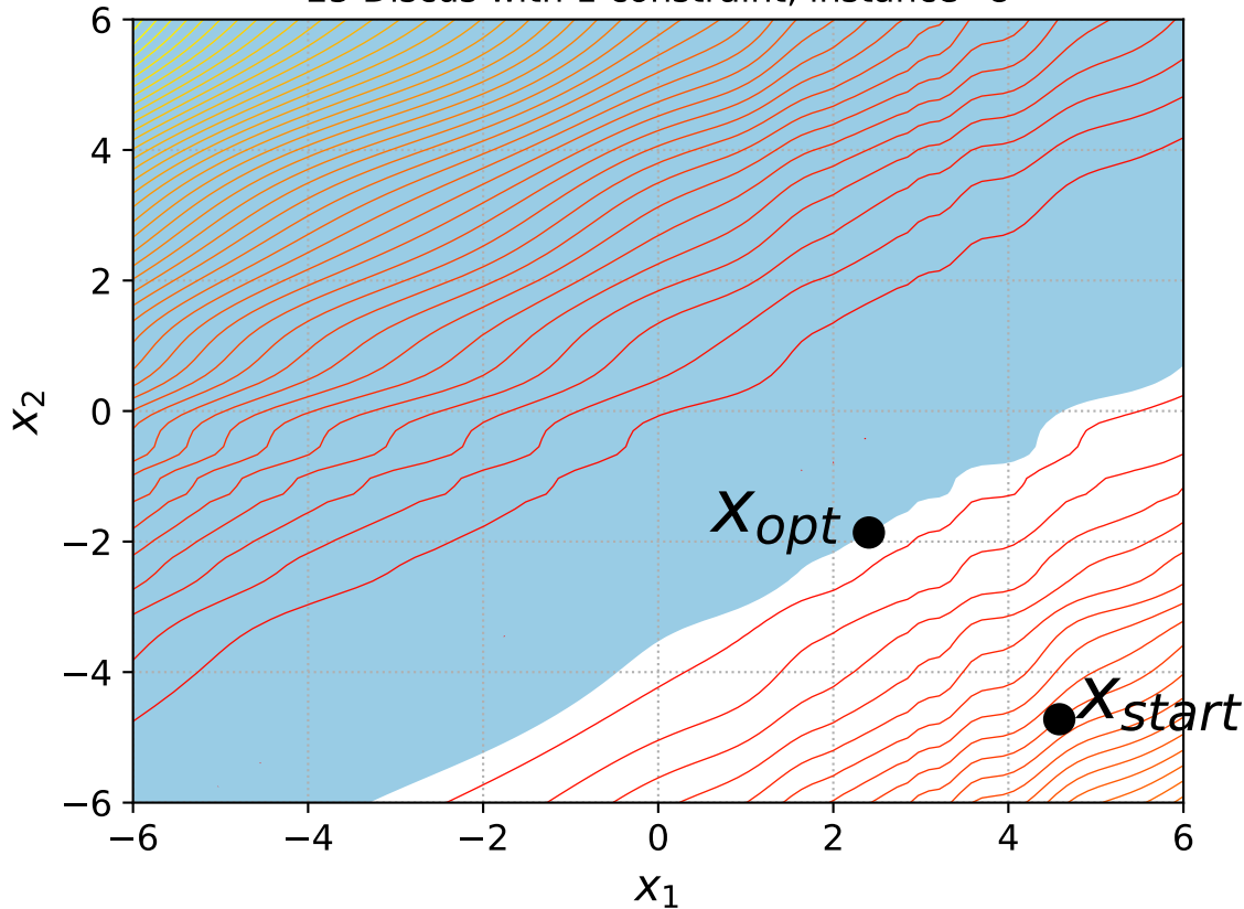
25 Discus with 1 constraint, instance=8
